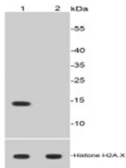
Fig. 1. Western blot analysis of Acetyl-Histone H2A (Lys9) on different cell lysates using anti-Acetyl-Histone H2A (Lys9) antibody at 1/500 dilution. Positive control: Lane 1: HeLa treated with 500 ng/ml Trichostatin A for 4 hours whole cell lysates; Lane 2: Untreated HeLa whole cell lysates
