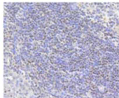
Fig. 2. Immunohistochemical analysis of paraffin-embedded human tonsil tissue using anti-Acetyl-Histone H2A (Lys9) antibody. Counter stained with hematoxylin.
